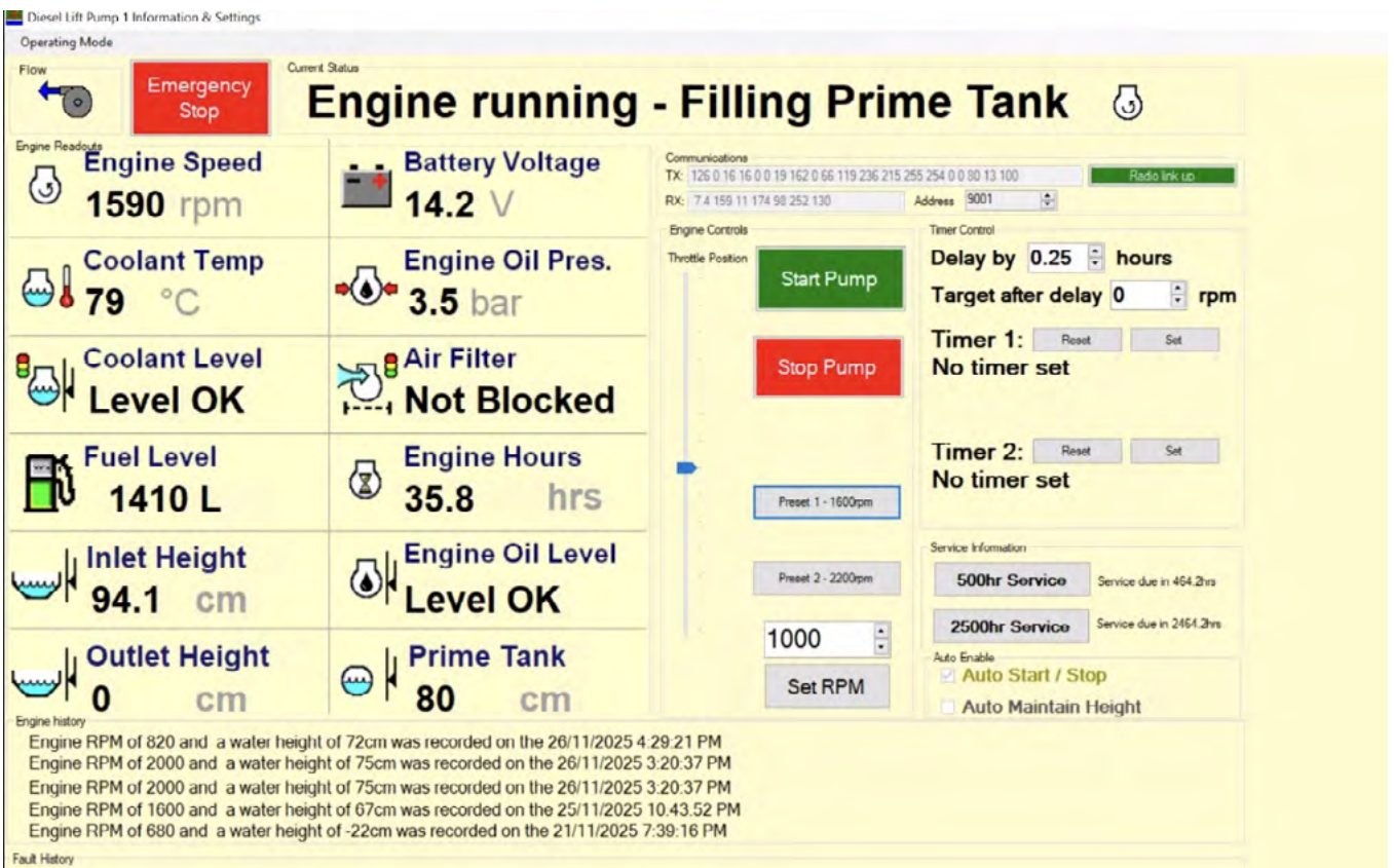
Figure 7: Top: Example of remote pump controller with manual override buttons. Bottom: Example of user interface for monitoring pumper operations.
